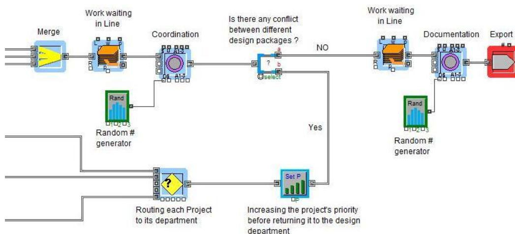
Figure 3: Modelling the finalisation and closing phase using 'Extend V.6'
