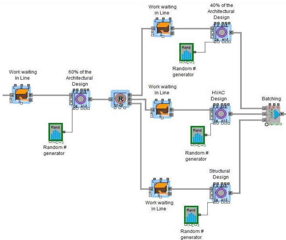
Figure 2: Modelling the core design phase using 'Extend V.6'
